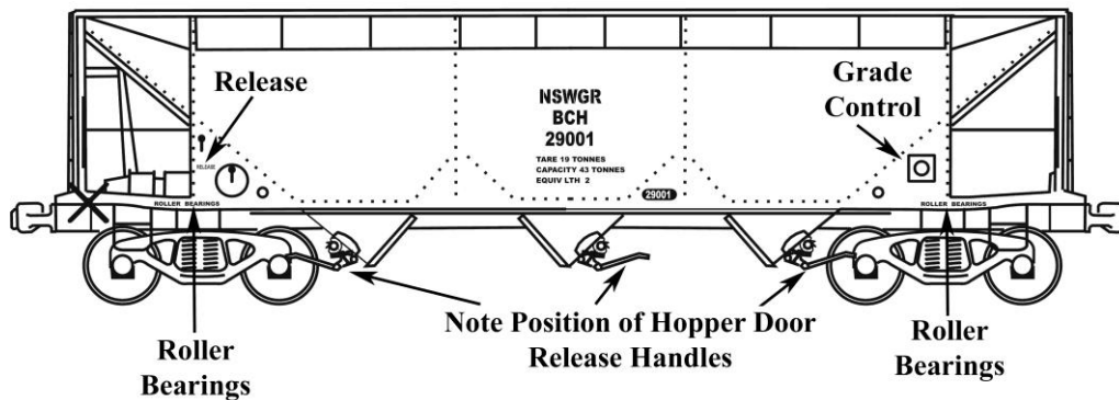
BCH Discharge Hopper Door Release Handles and Decal Location Diagram
